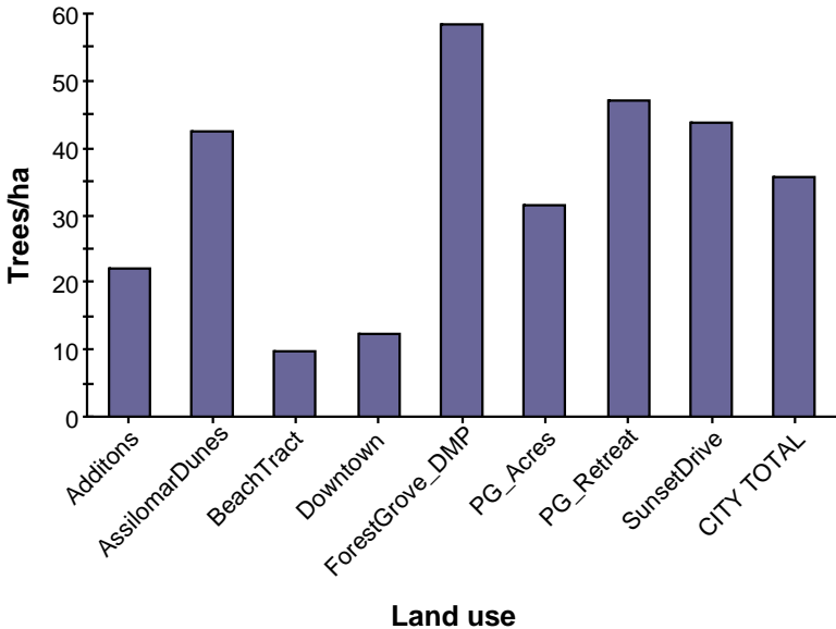
Figure 2. Number of trees/ha in City of Pacific Grove by land use
