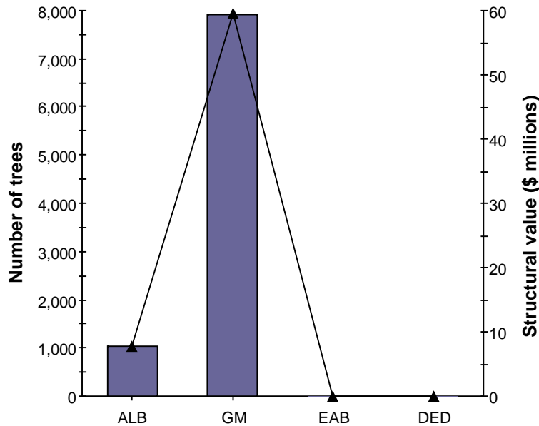
Figure 9. Number of susceptible City of Pacific Grove trees and structural value by pest (line graph is structural value)
