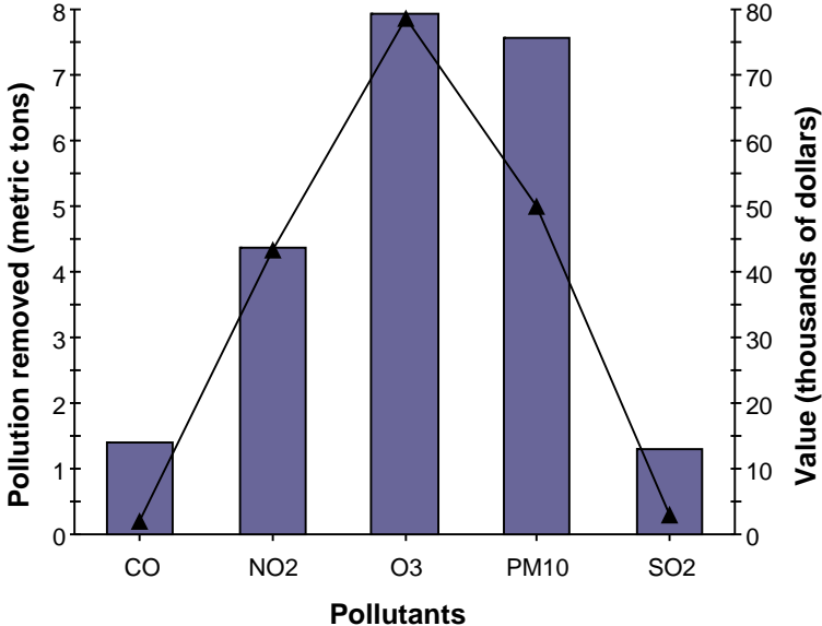
Figure 6. Pollution removal and associated value for trees in City of Pacific Grove (line graph is value)
