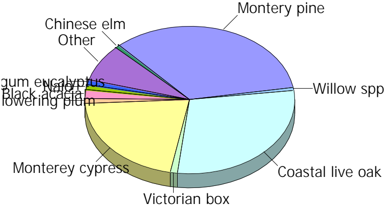
Figure 1. Tree species composition in City of Pacific Grove
