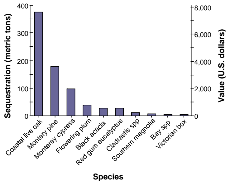
Figure 7. Carbon sequestration and value for species with greatest overall carbon sequestration in City of Pacific Grove
