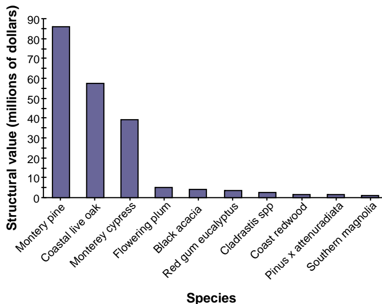
Figure 8. Structural value of the 10 most valuable tree species in City of Pacific Grove
